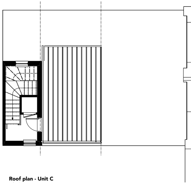
Roof plan - Unit C
