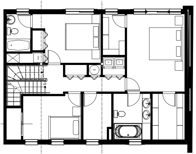
Second Floor plan - Unit C
