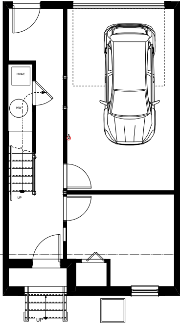
First Floor plan - Unit A
