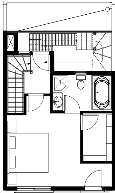
Fourth Floor Plan - Unit A
