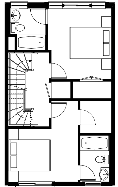
Third Floor plan - Unit A
